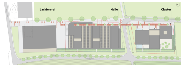
Situationsplan
