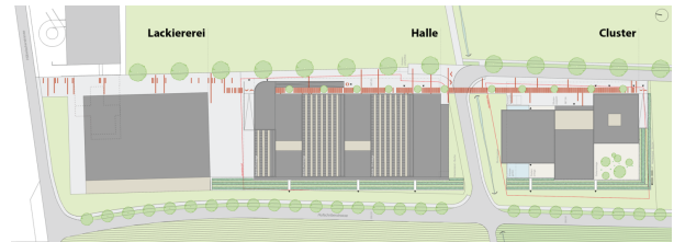
Situationsplan
